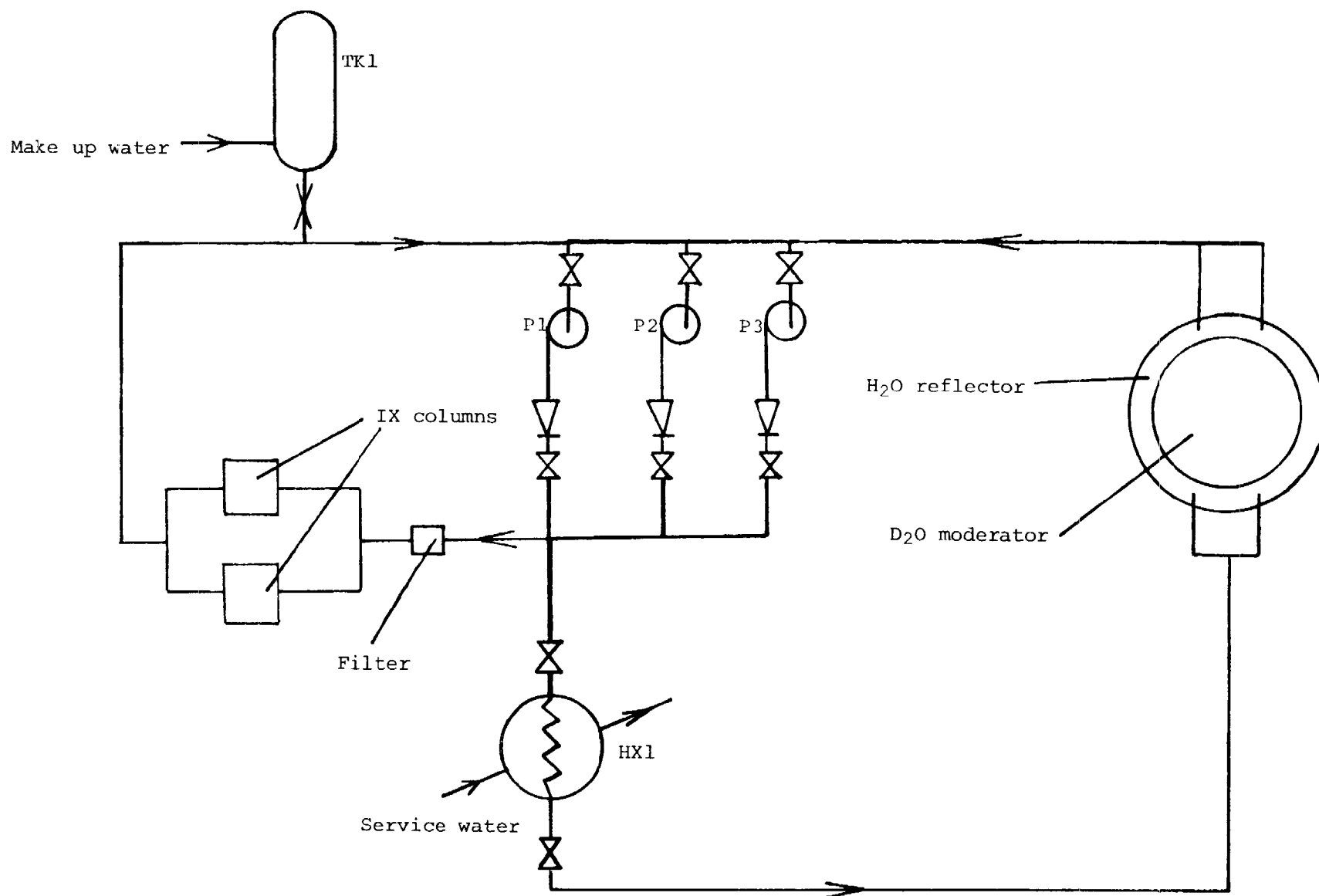
Figure 1: Reflector System NPD
