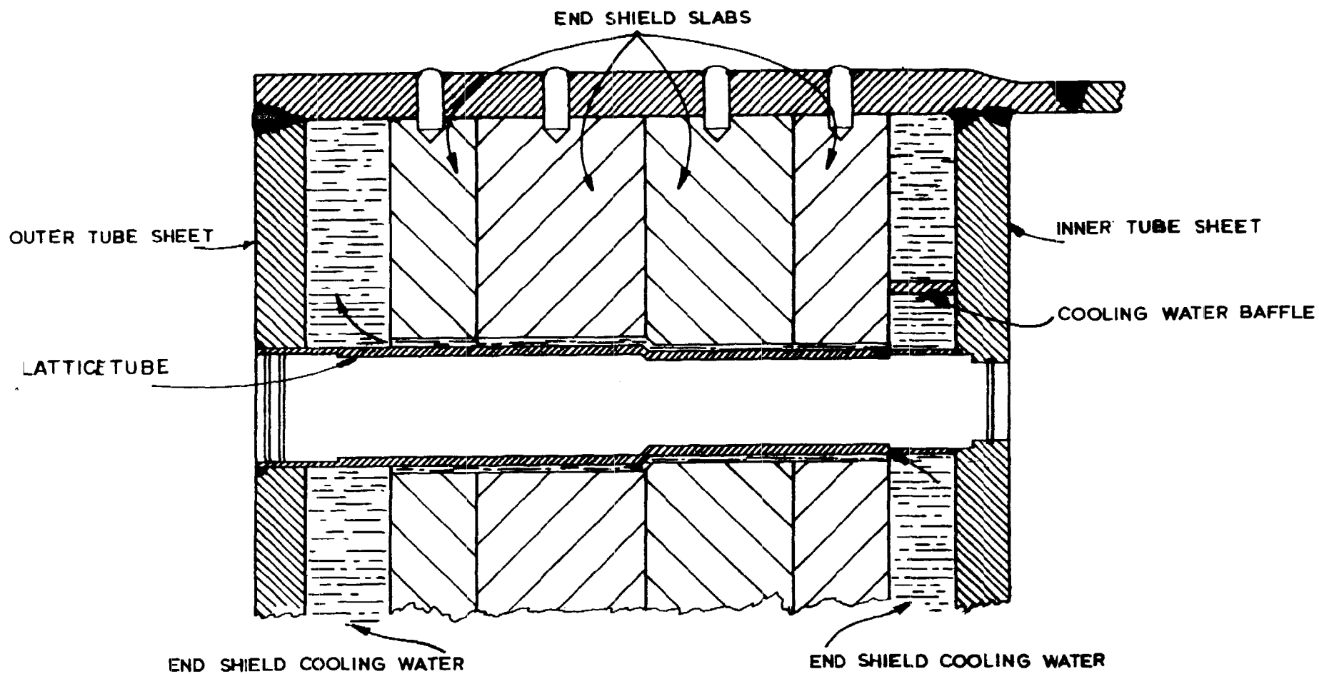
Figure 4: Pickering GSA End Shields
